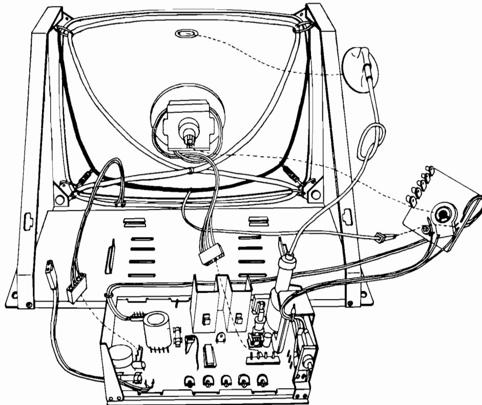
Figure 1 Overview of Disco 19-Inch Color Raster Display
