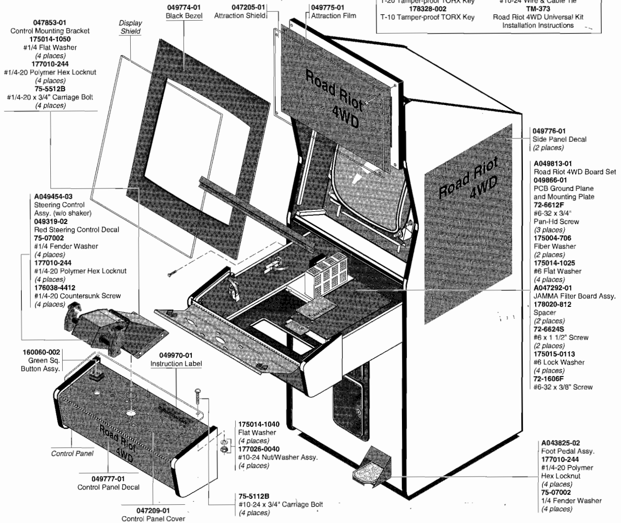
Control panel in closed position
