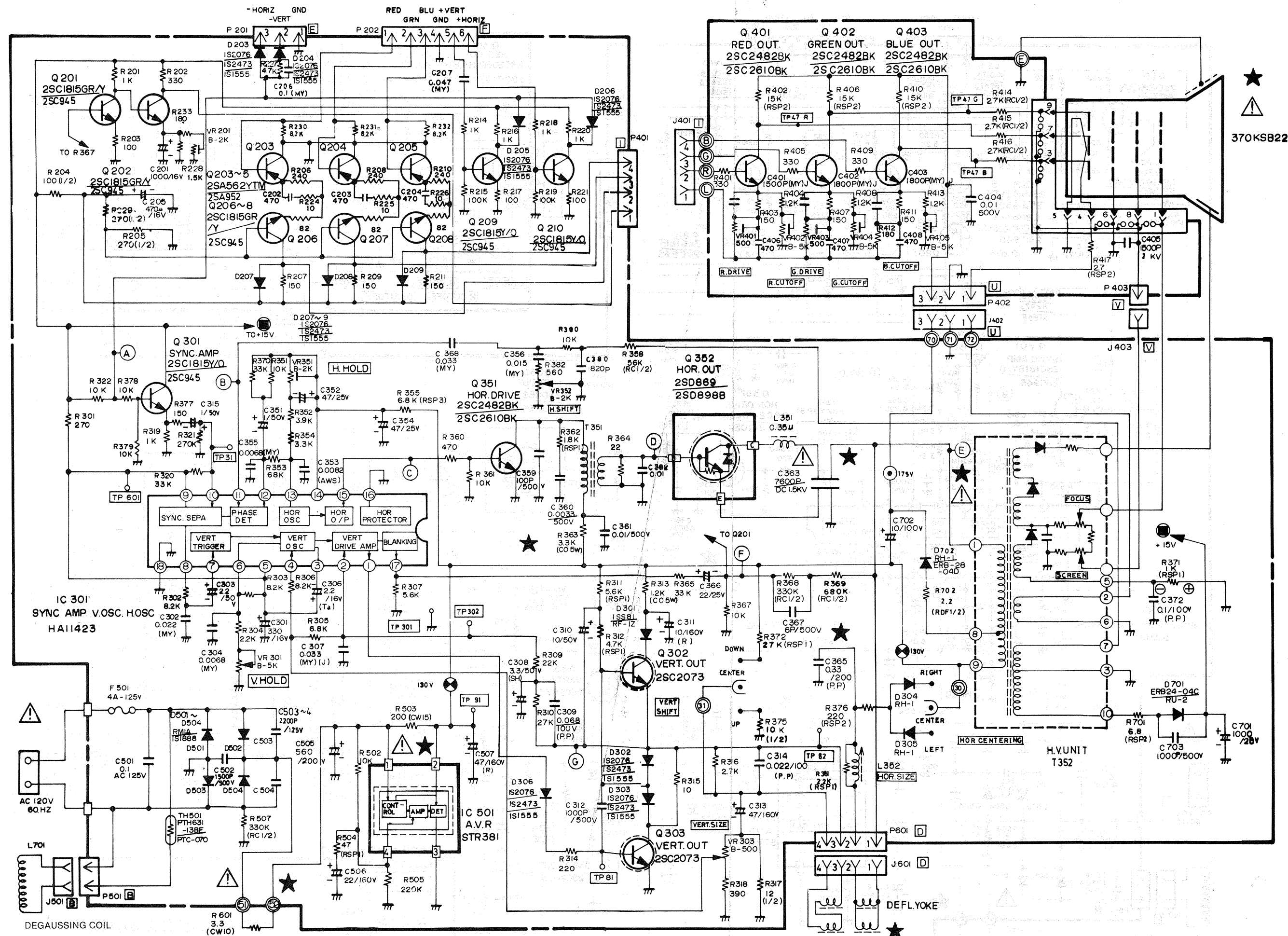
13" MONITOR SCHEMATIC
