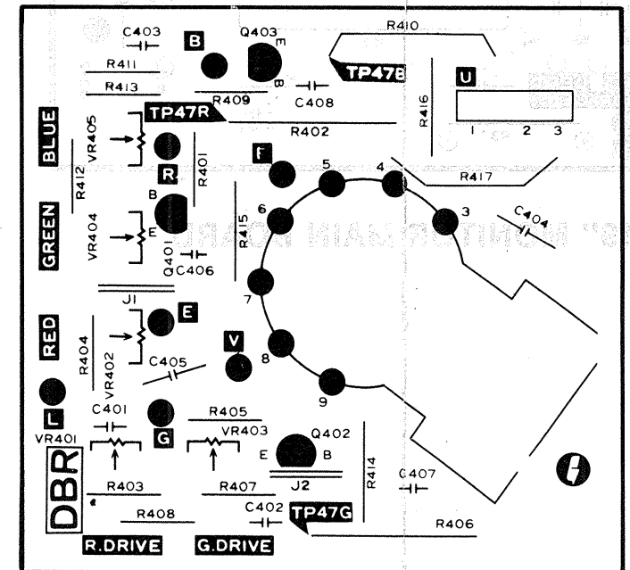
13" MONITOR NECKBOARD
