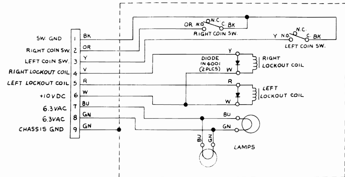
Upright and Cabaret Coin Door Wiring Diagram
