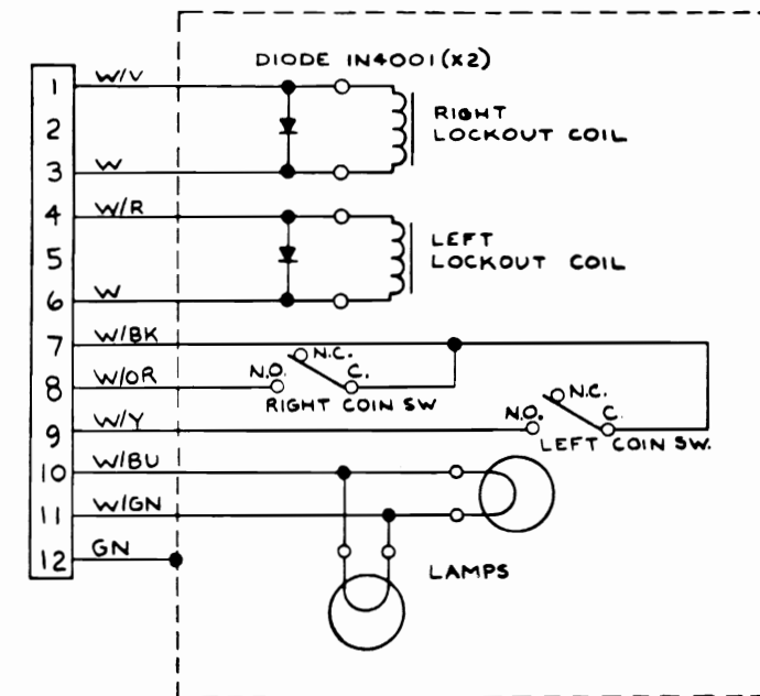
Cocktail Coin Acceptor Wiring Diagram
