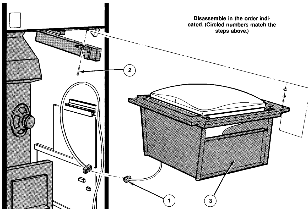
Figure 12 Monitor Removal
