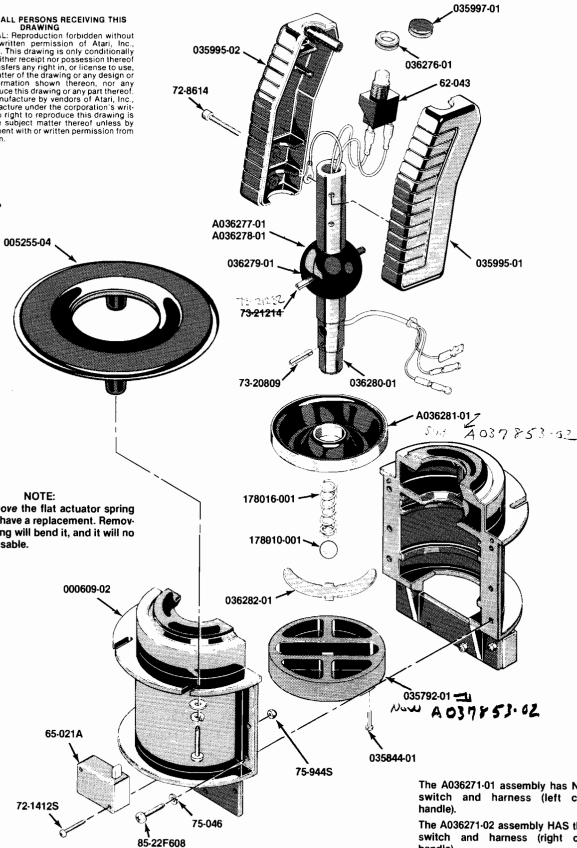
Figure 21 Control Handle Assembly A036271-01 and -02 B
