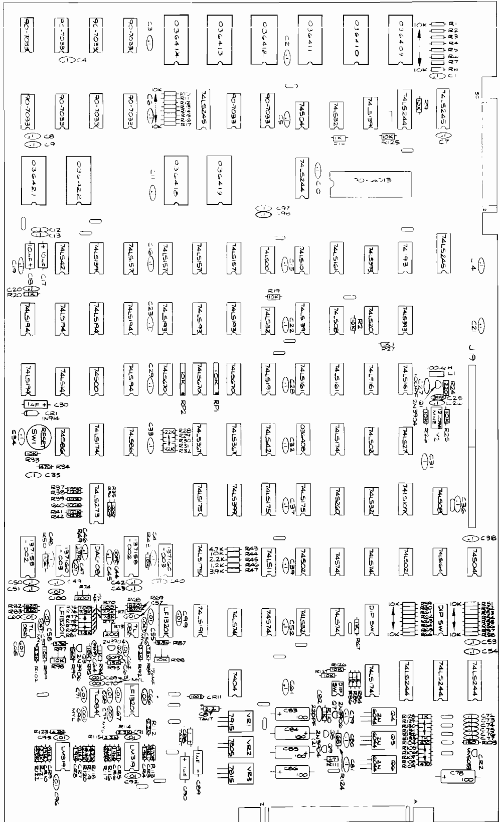
Figure 26 Battlezone™ Analog Vector-Generator PCB Assembly A036424-02 A
