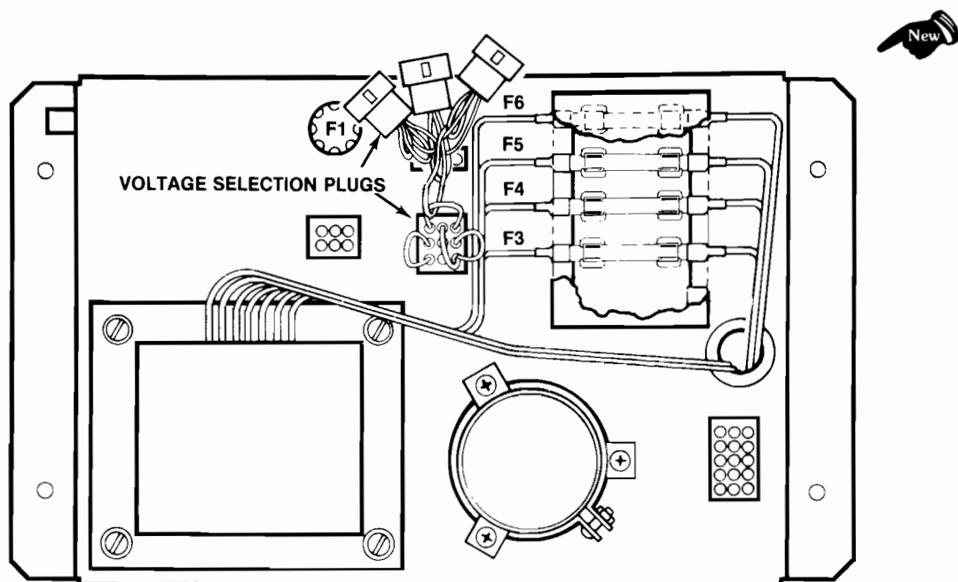
Figure 3 International Line Voltage Selection
