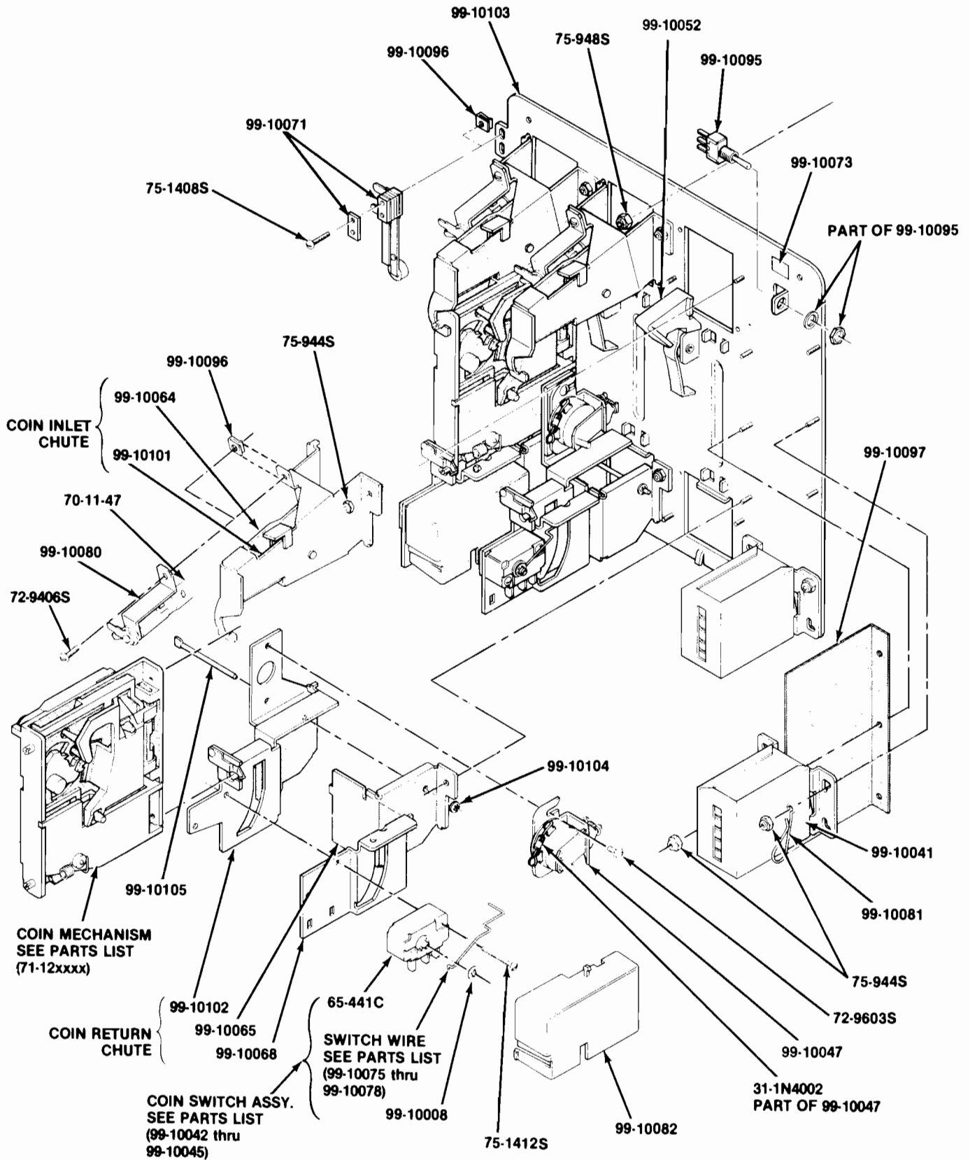
Figure 28 New Coin Door 71-10xxxx D
