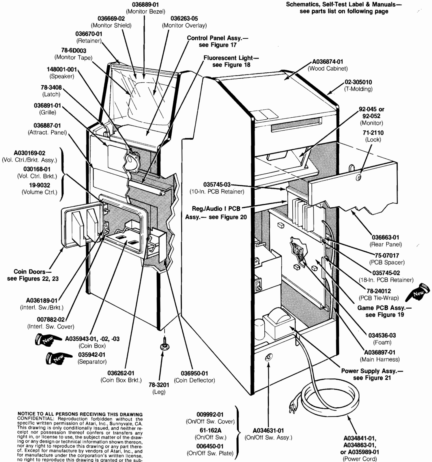
Figure 16 Cabinet-Mounted Assemblies A036873-xx A
