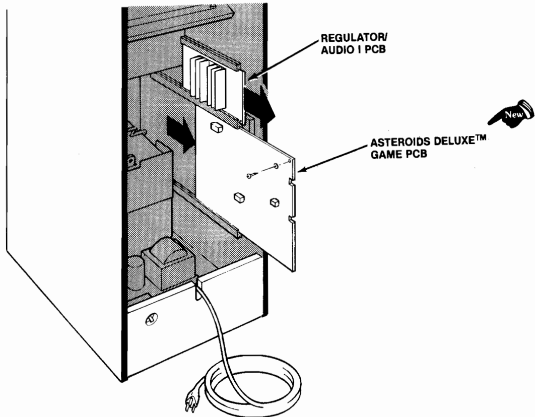
Figure 12 Printed-Circuit Board Removal
