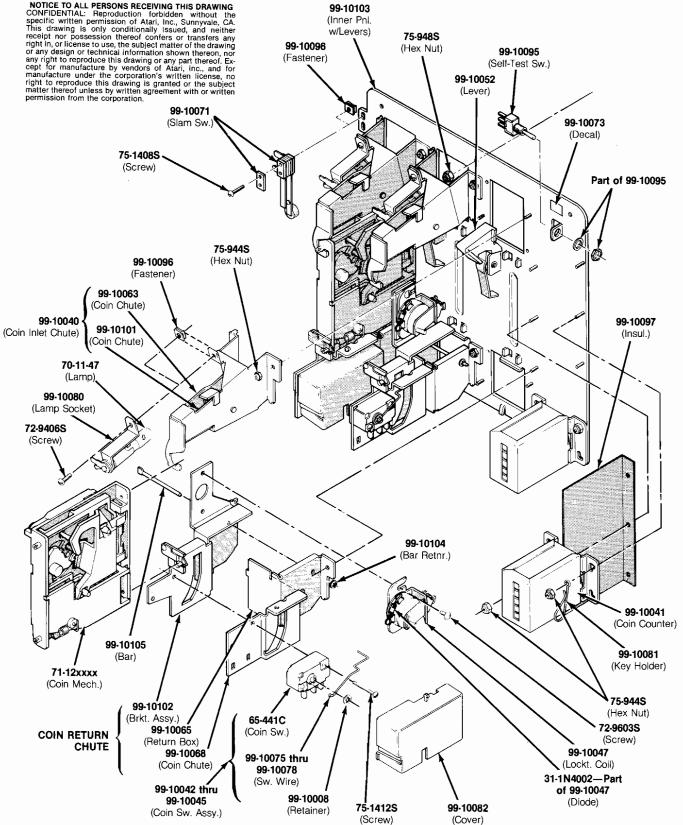
Figure 22 American-Made Coin Door 71-10xxxx D
