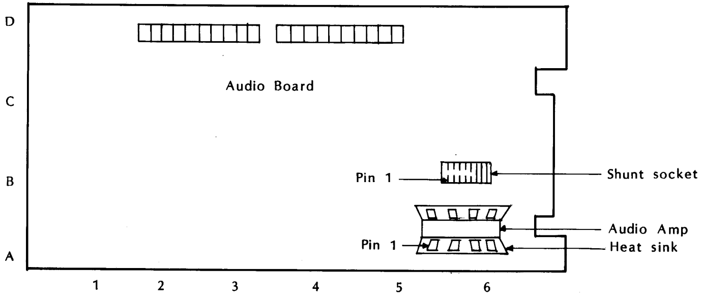
Shunt for LM377, LM378
