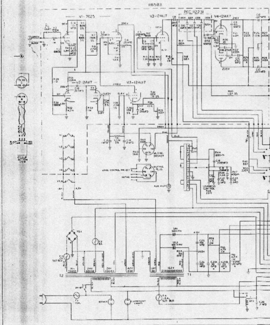
Fig. 94. 540 Sound System Schem
