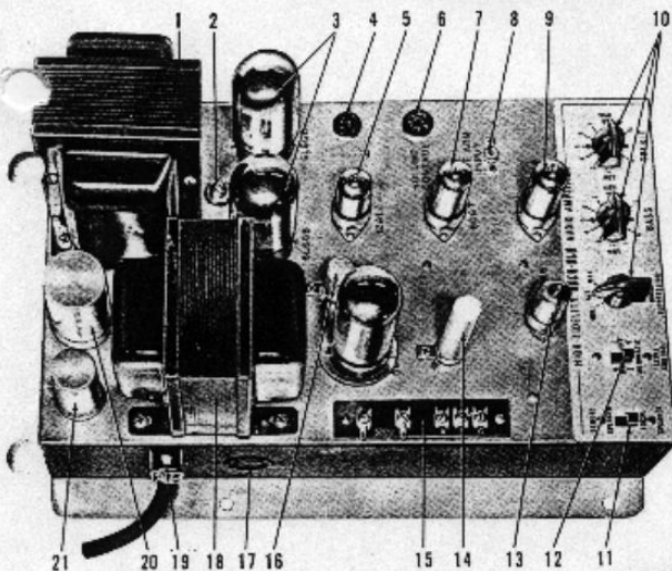
No. 30625-A Amplifier Assembly (Less Tubes)
