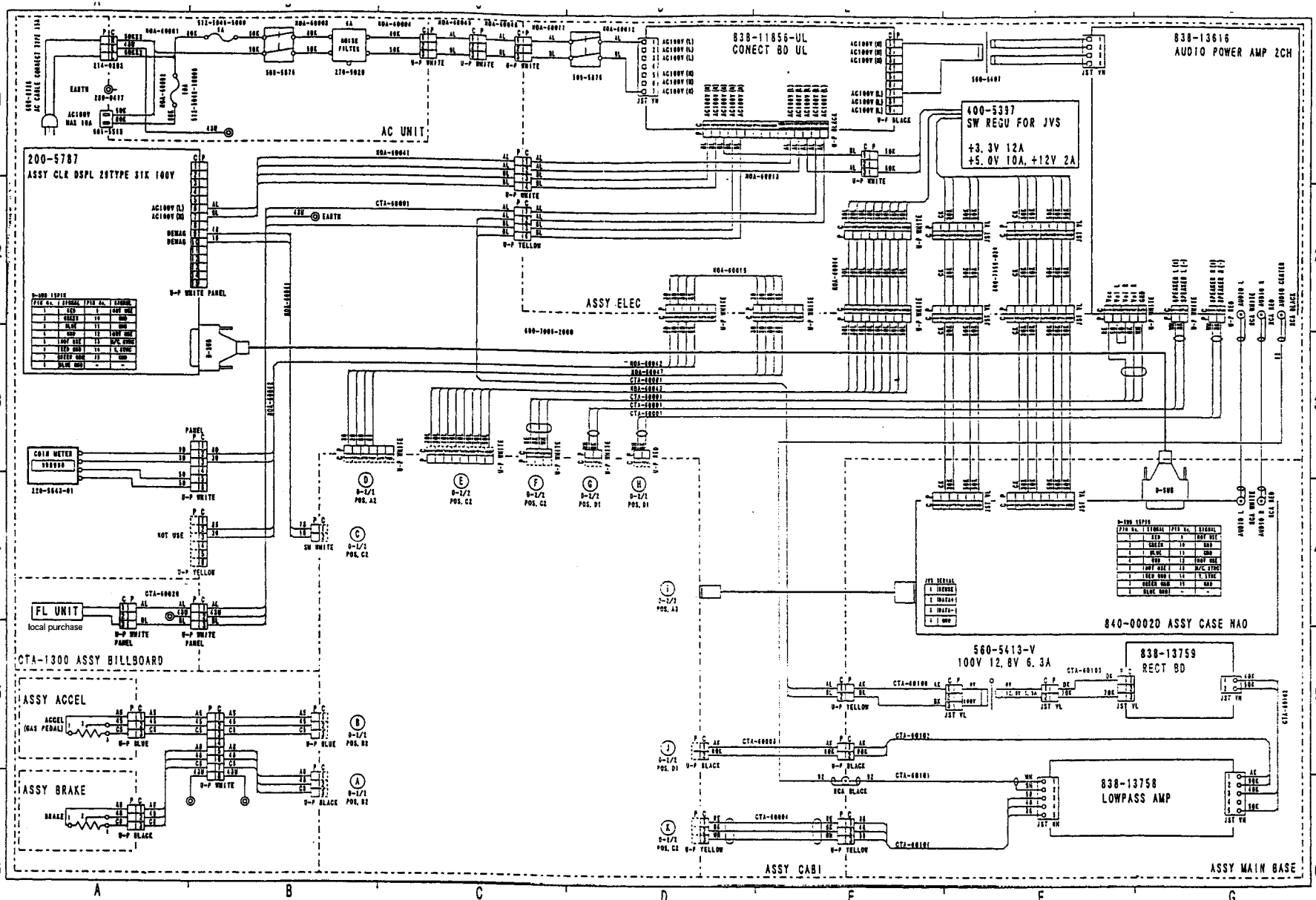
Wiring Diagram (D-1/2)
